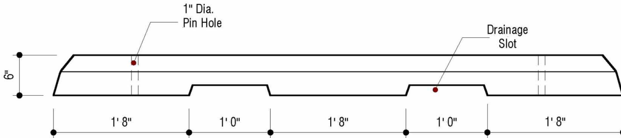
FRONT ELEVATION
