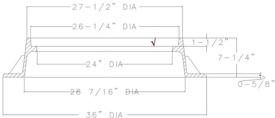
1.030703;FRAME SECTION
