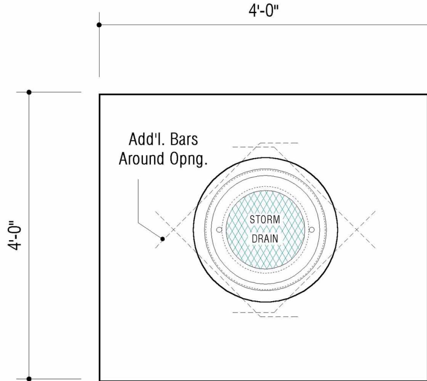
TOP SLAB PLAN
