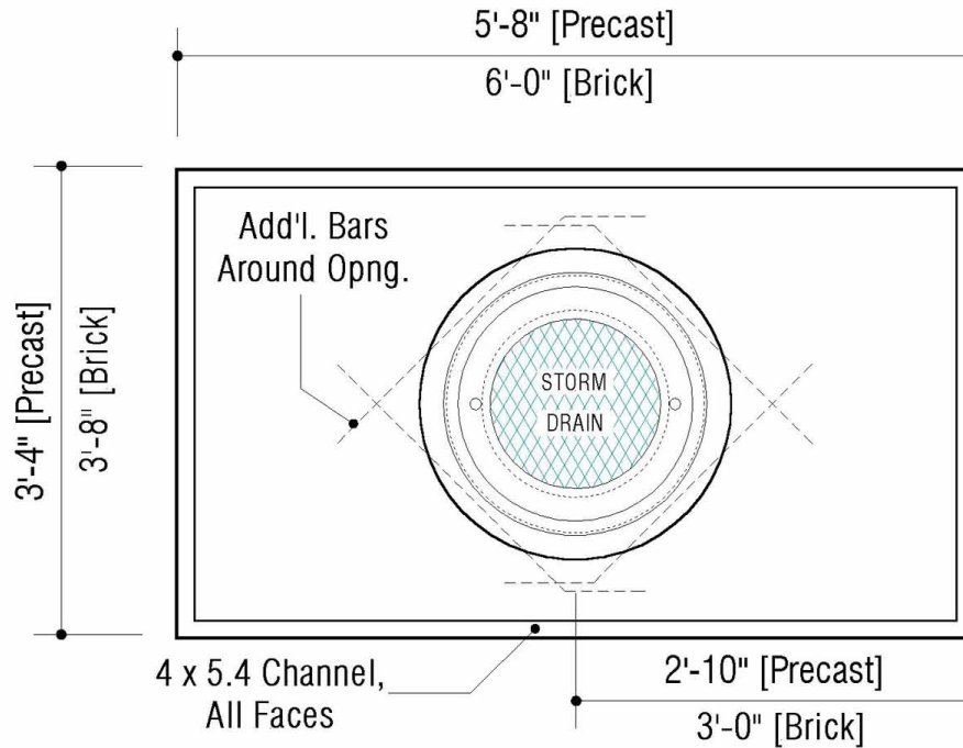
TOP SLAB PLAN
