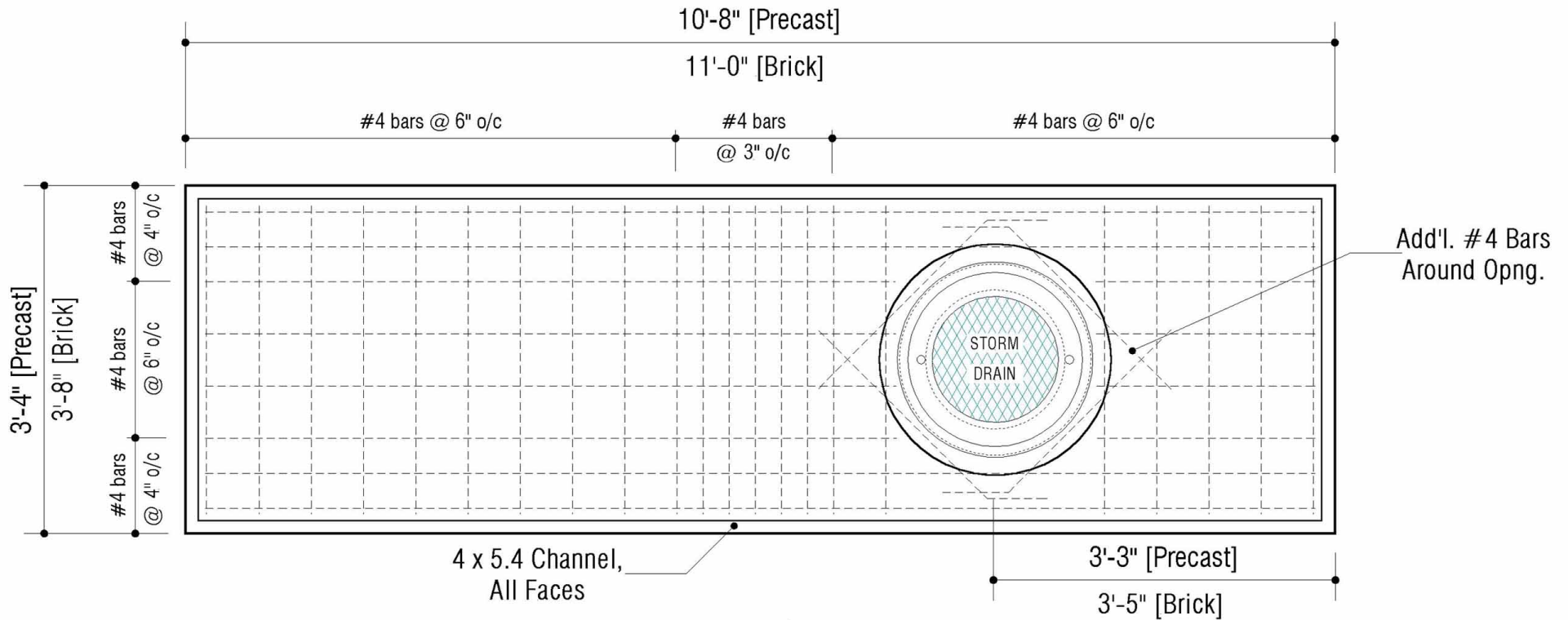
TOP SLAB PLAN
