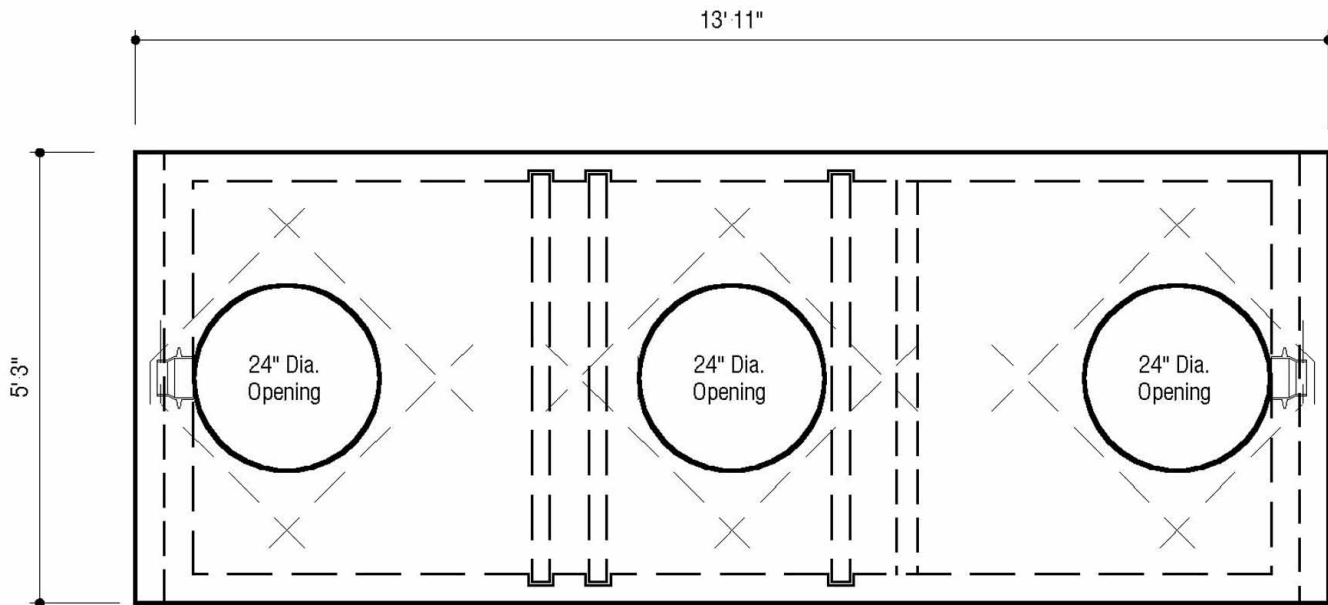
PLAN VIEW
