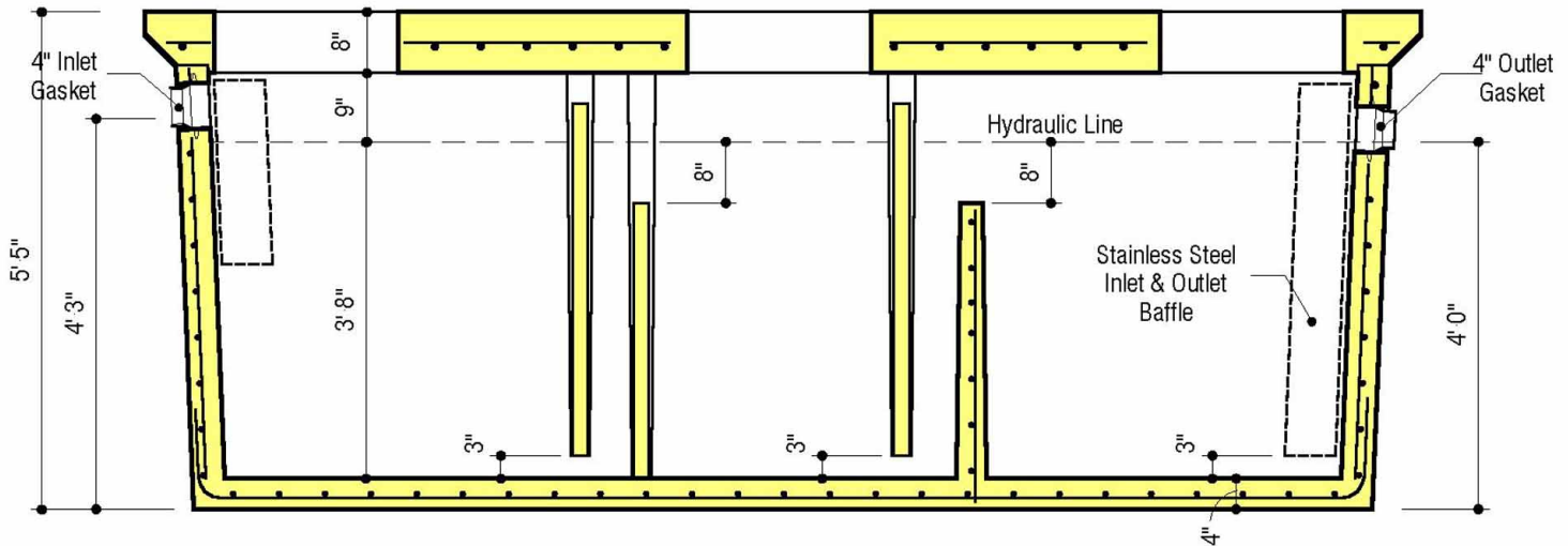
SECTION VIEW
