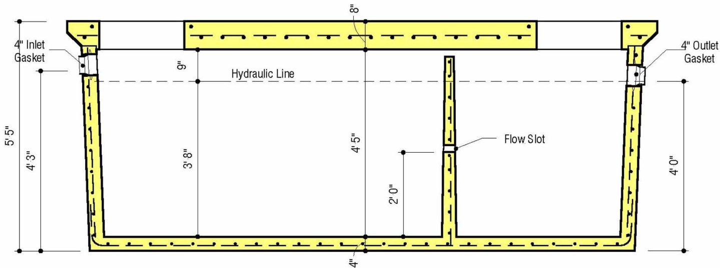
SECTION VIEW
